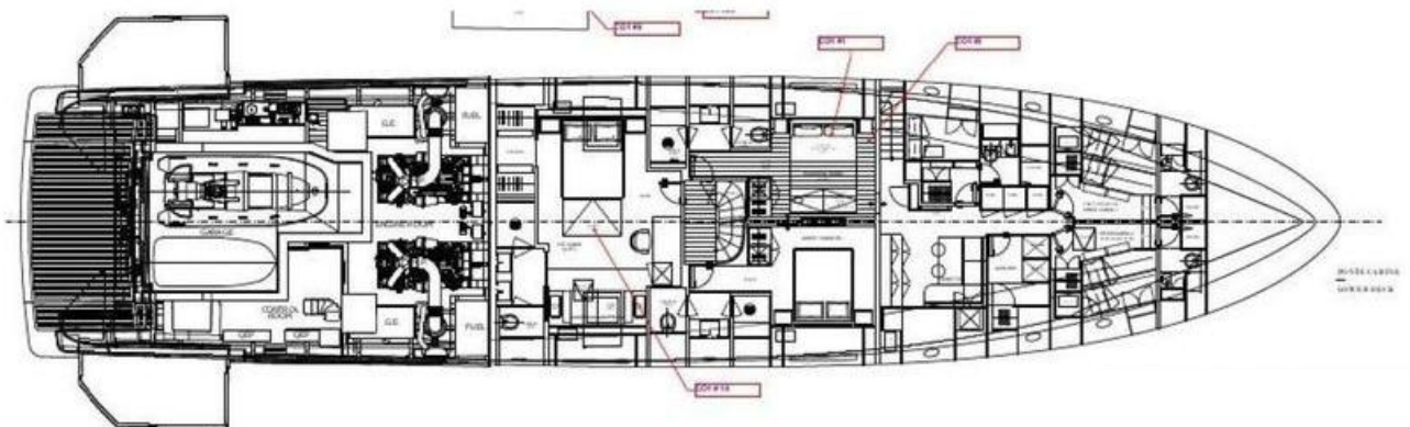
LOWER DECK
